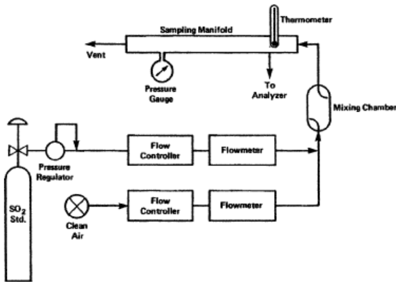
Figure 2. Calibration system using a compressed gas standard.
