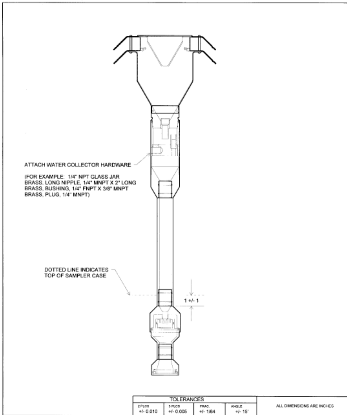
FIGURE L-1. PM 2.5 SAMPLER, ASSEMBLY
